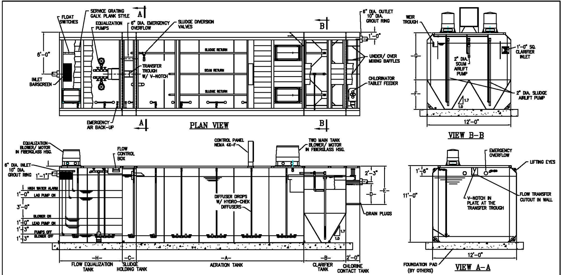
ELEVATION VIEW w/o SIDE WALL
